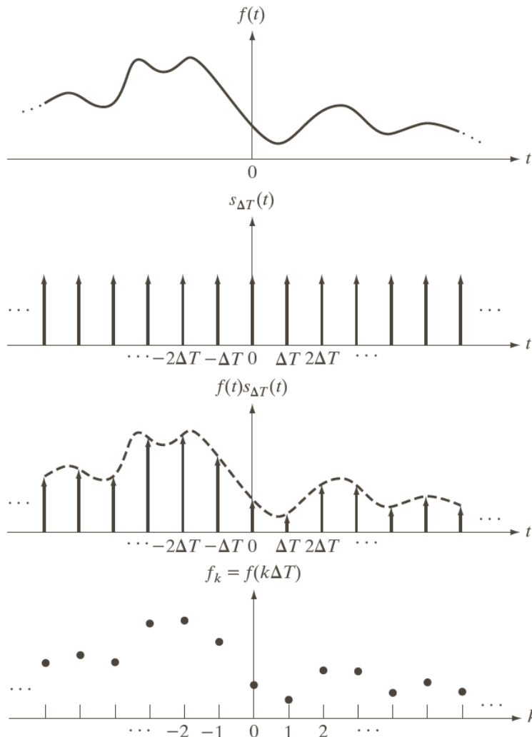
a b c d FIGURE 4.5 (a) A continuous function. (b) Train of impulses used to model the sampling process. (c) Sampled function formed as the product of (a) and (b). (d) Sample values obtained by integration and using the sifting property of the impulse. (The dashed line in (c) is shown for reference. It is not part of the data.)
