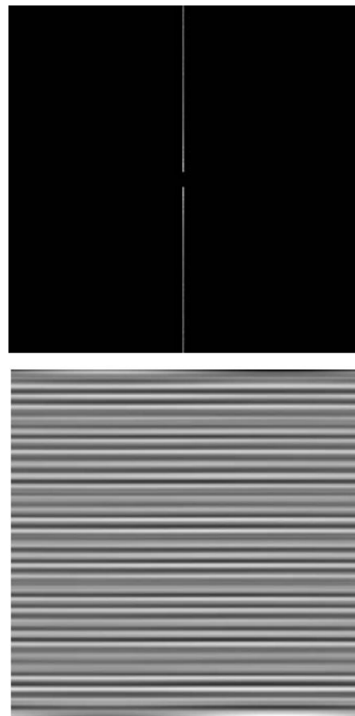
a b FIGURE 4.66 (a) Result (spectrum) of applying a notch pass filter to the DFT of Fig. 4.65(a). (b) Spatial pattern obtained by computing the IDFT of (a).
